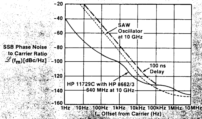
Figure 5.3. Typical HP 11729C sensitivity with a 100 ns delay line.
