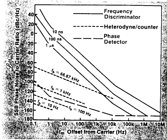
Figure 3.2. Comparison of typical system sensitivities at 10 GHz.
