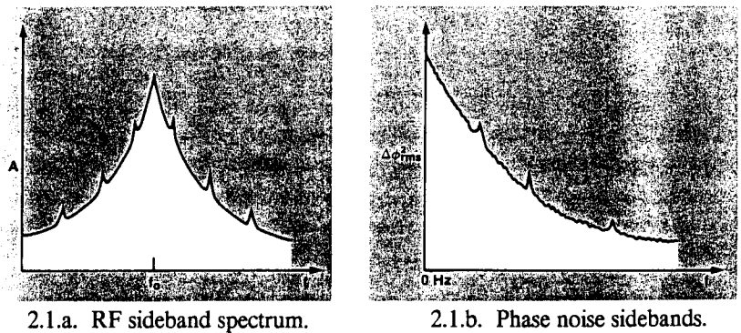
Figure 2.1. CW Signal sidebands viewed in the frequency domain.
