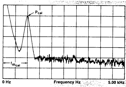
Figure 5.6. System response to calibration signal.
