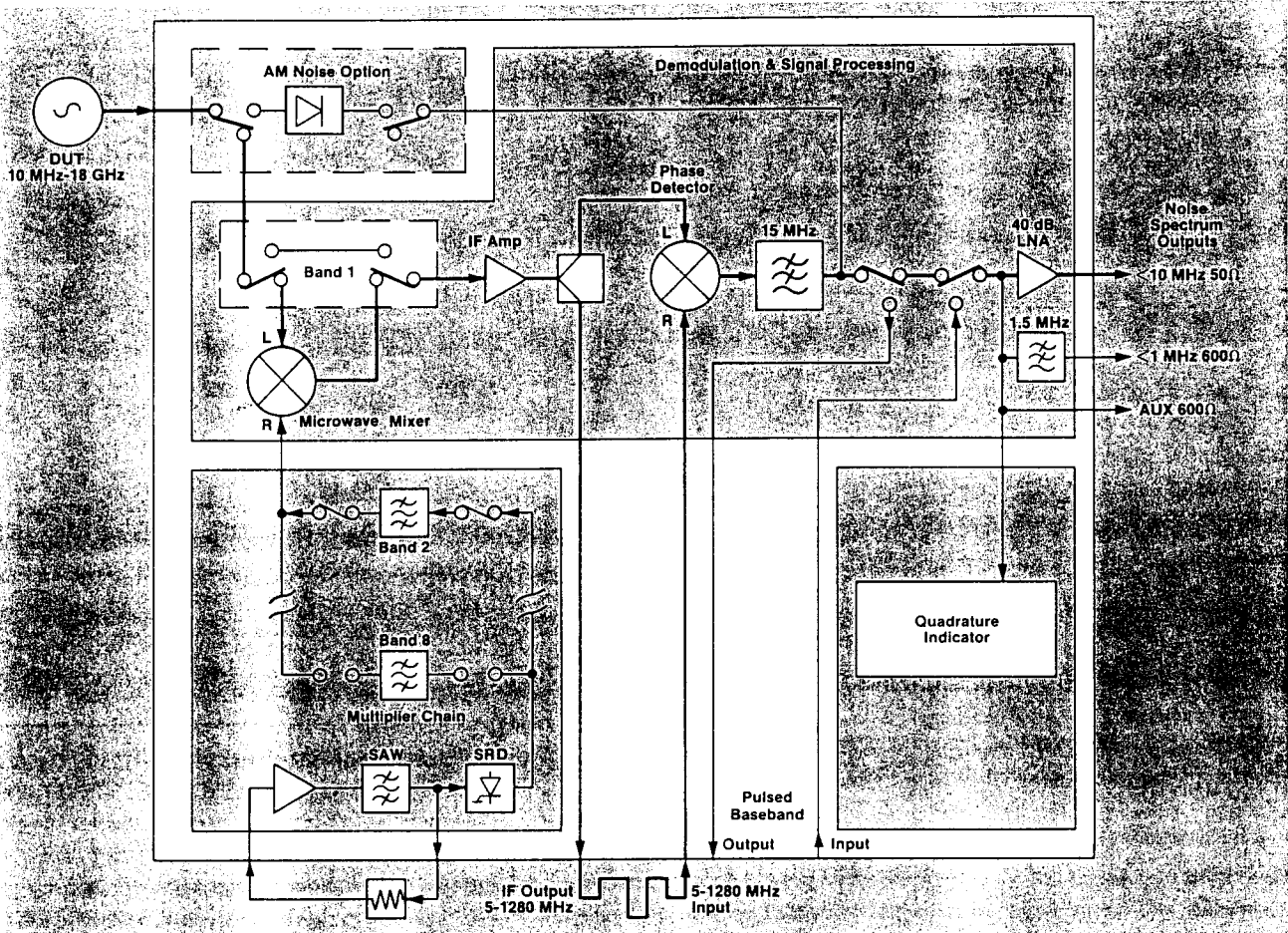
Figure 4.4. HP 11729C Carrier Noise Test Set.
