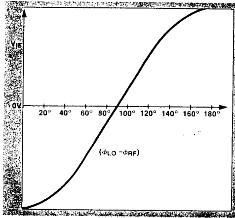
Figure B.1. Typical double-balanced mixer phase detector characteristic.
